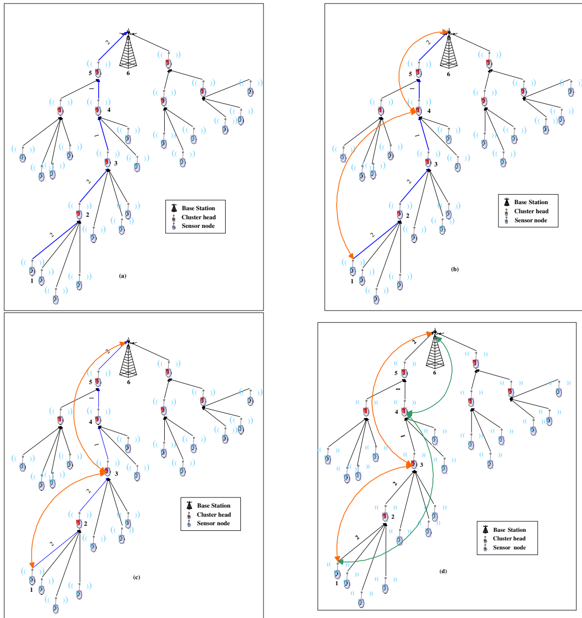
Fig. 1. (a) Information dissemination tree representation of a multi-layered wireless sensor network with a five-hop path from Node 1 (source) to Node 6 (sink). (b) A two-hop path that bypasses certain layers from Node 1 to Node 6. (c) Another two-hop path that also bypasses layers from Node 1 to Node 6. (d) Two node-disjoint paths between Node 1 to Node 6 with a maximum of two hops for enhanced loss-tolerance given a delay-constraint.
